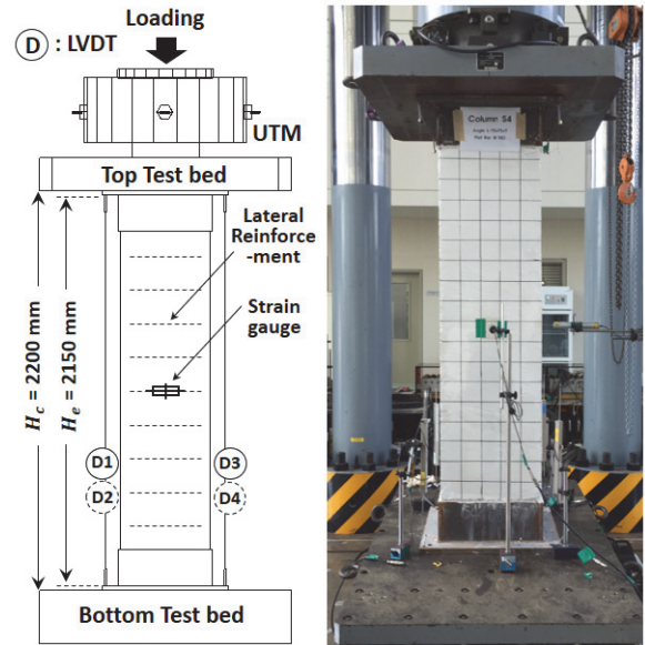
Fig. 4. Test set-up
