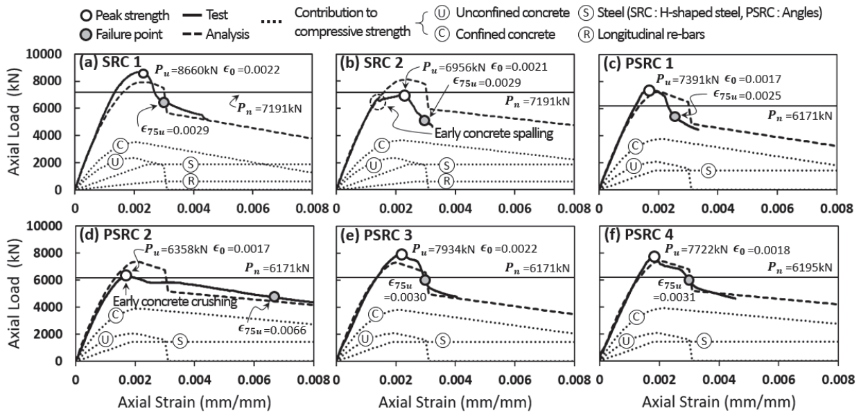
Fig. 6. Axial load - strain relationships of test specimens
