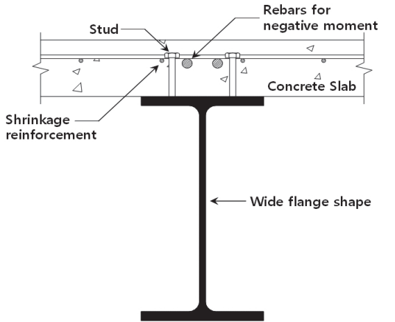
(a) Wide flange composite beam
