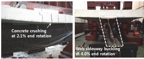
(a) Ho-H
