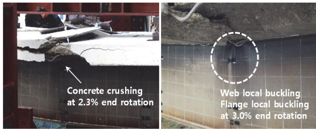
(b) Ho-U
