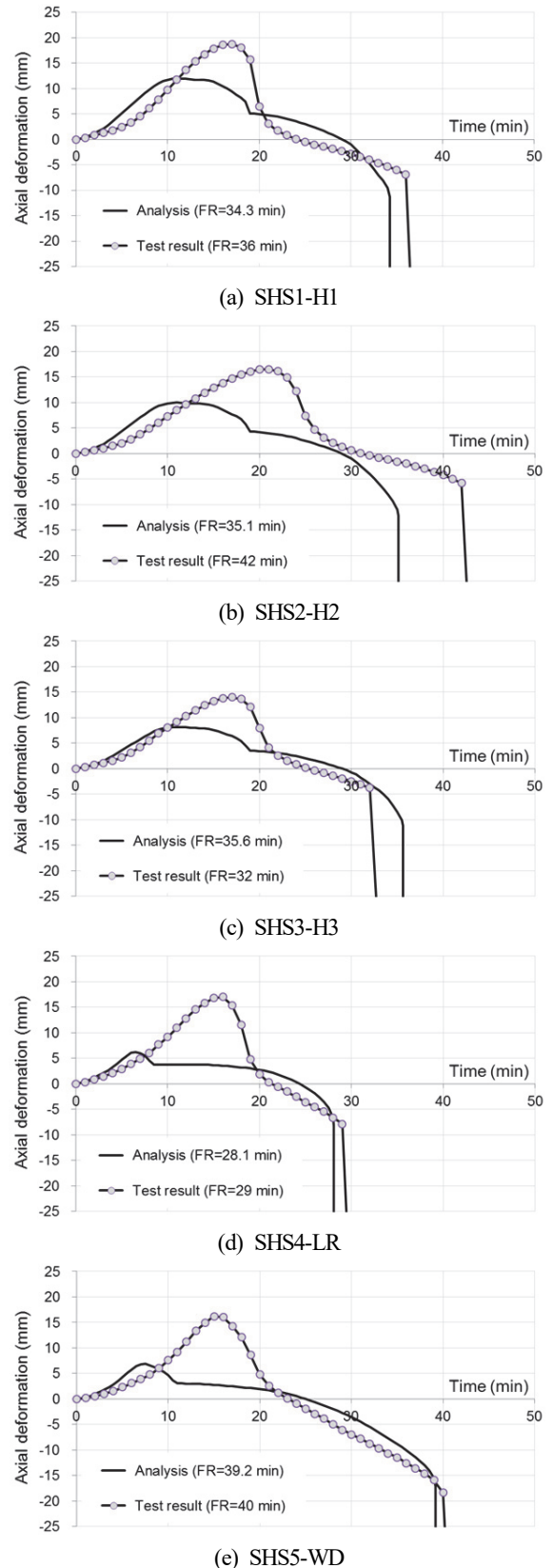
Fig. 10. Comparison of axial deformations between simulation and test
