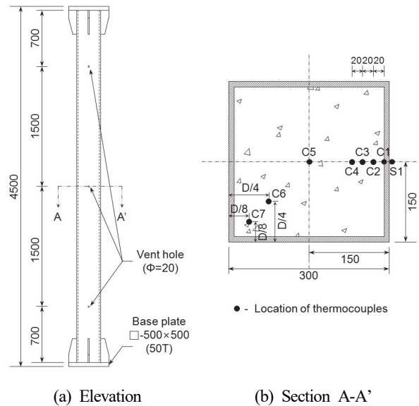
Fig. 2. Specimen details and location of thermocouples
