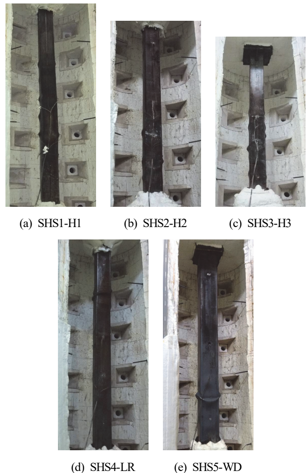
Fig. 8. Specimens after fire test
