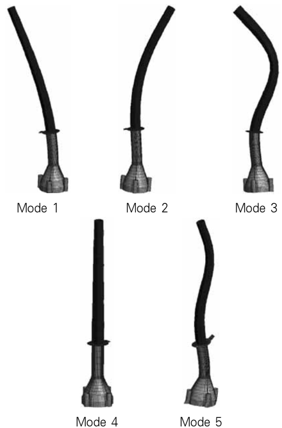
Fig. 14 First 5 eigen mode shapes
