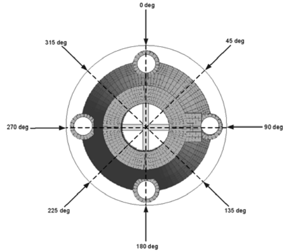
(a) Load direction cases
