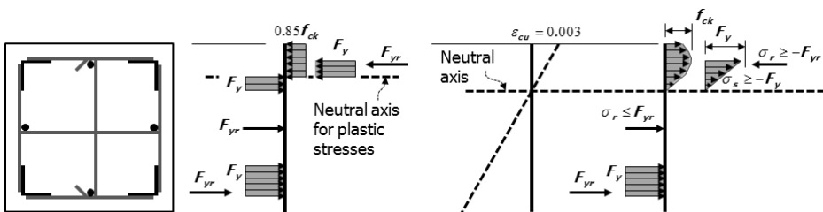
(a) Method I: Plastic stress distribution (b) Method II: Strain-compatible stress distribution
