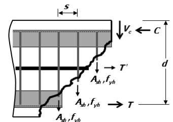
Fig. 3 Shear strength
