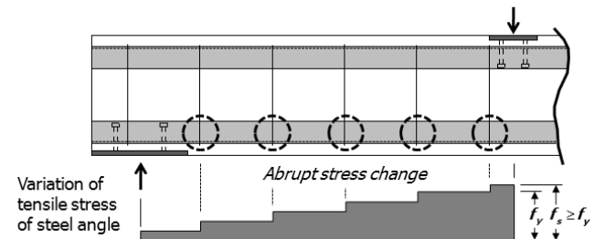
Fig. 11 Stress Concentration at Weld Joints Between Angle and Lateral Re-bars
