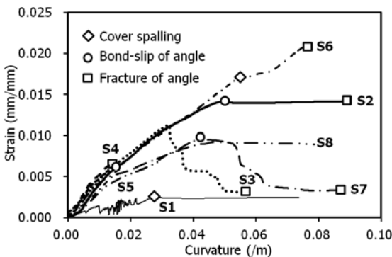
Fig. 9 Longitudinal Strains of Steel Sections
